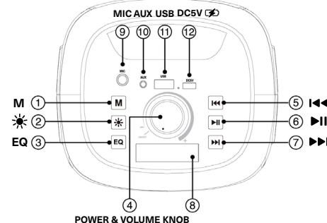
POWER & VOLUME KNOB
