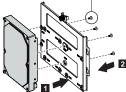
HDD Screw
