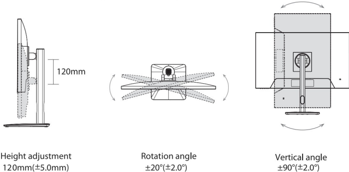
Figure 2-2 Monitor Adjustments
